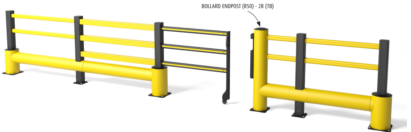
EXAMPLE SET UP FOR A SLIDING GATE TB400 PLUS IN COMBINATION WITH A BOLLARD
